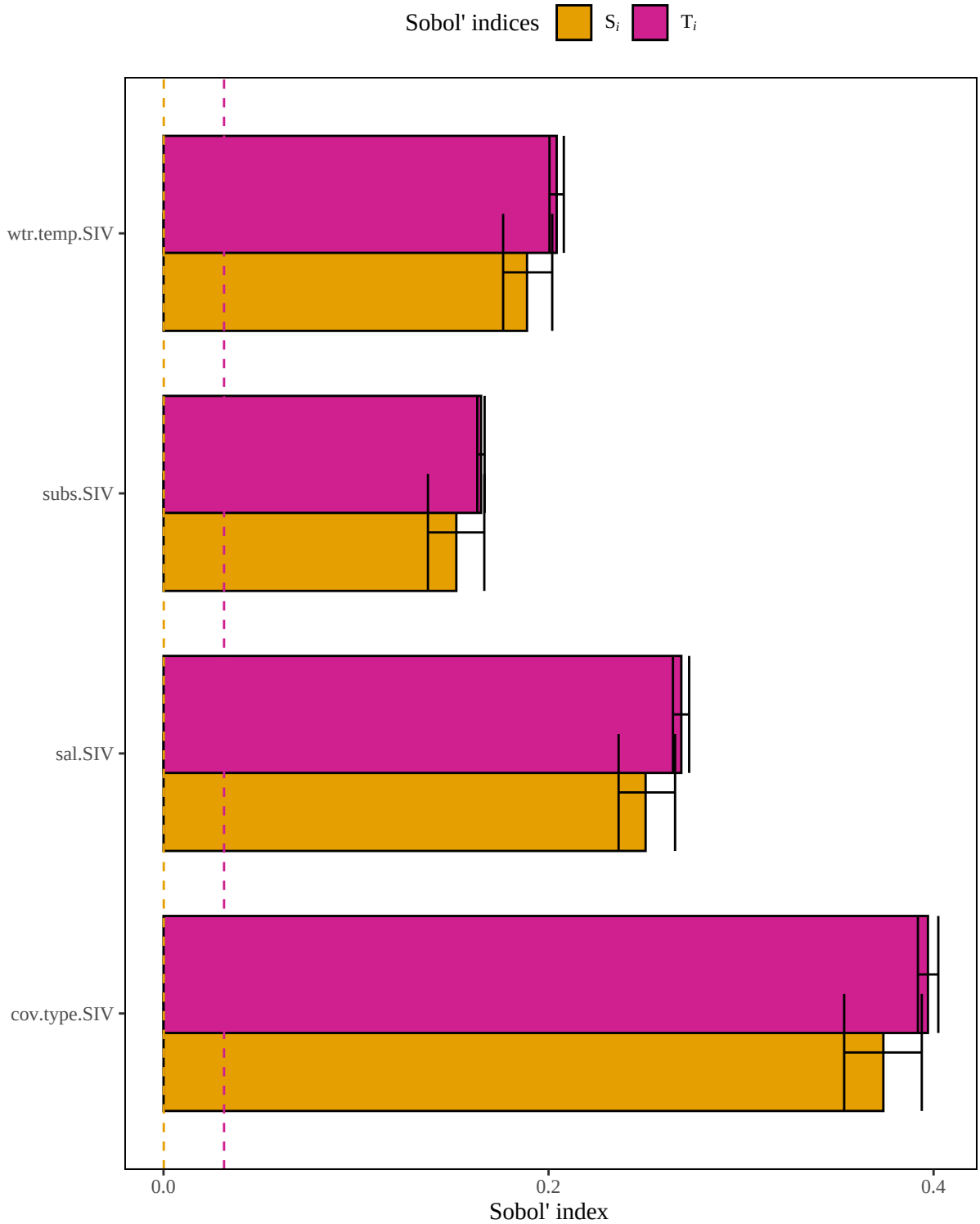
Figure 5. Results of a sensitivity analysis for the pinkshrimpSeagrassVeg model based on a geometric mean structure. Dashed lines represent baseline numerical approximation error for S_i and T_i ( i.e. , dummy variables).
