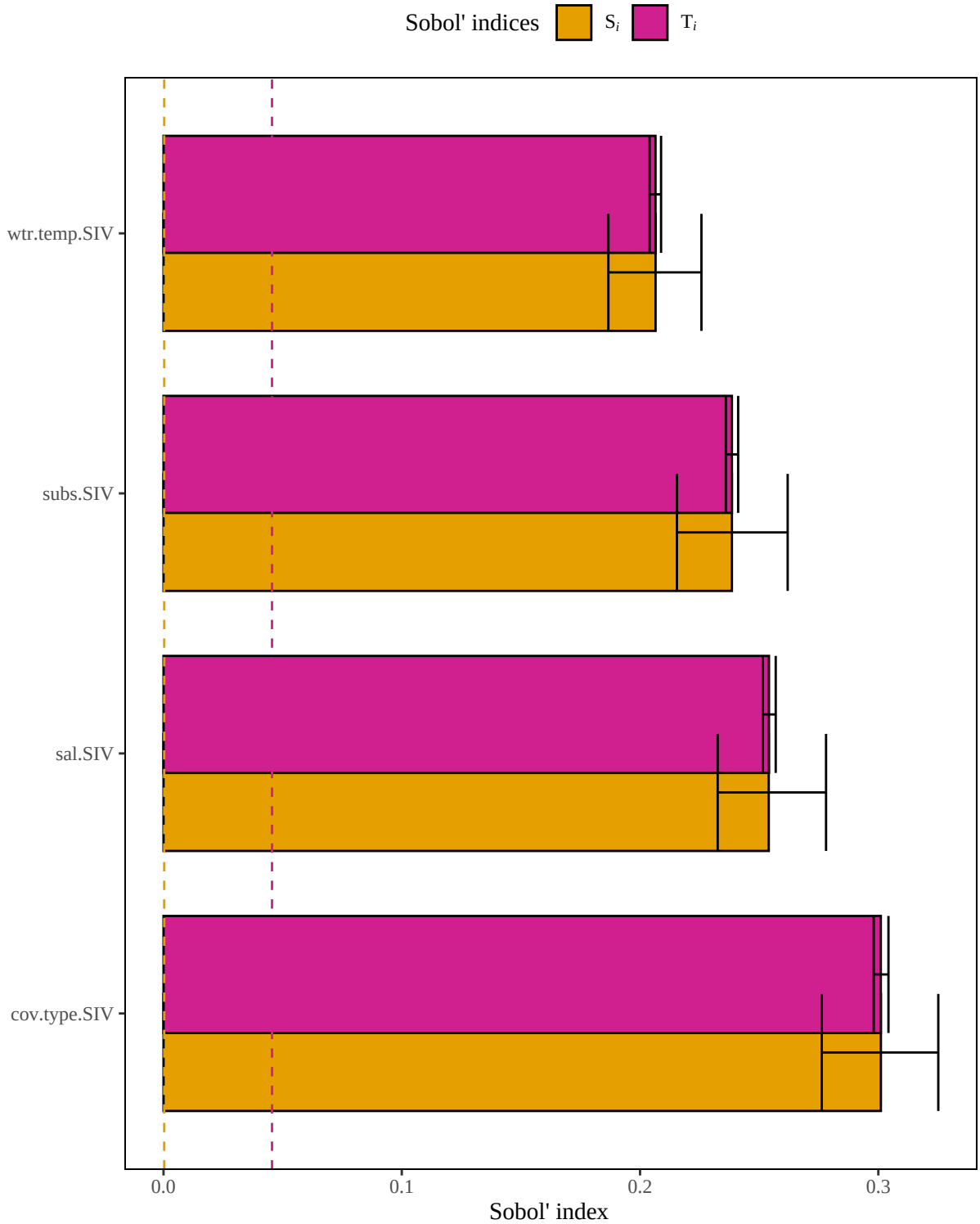
Figure 4. Results of a sensitivity analysis for the pinkshrimpSeagrassVeg model based on an arithmetic mean structure. Dashed lines represent baseline numerical approximation error for S_i and T_i ( i.e. , dummy variables).
